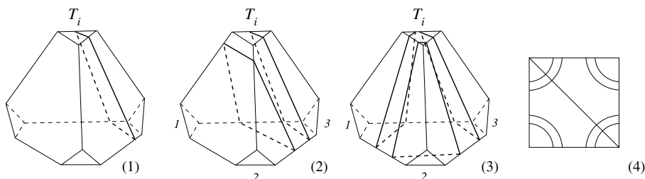
Figure 3: Types of intersection between a normal surface and a tetrahedron.
