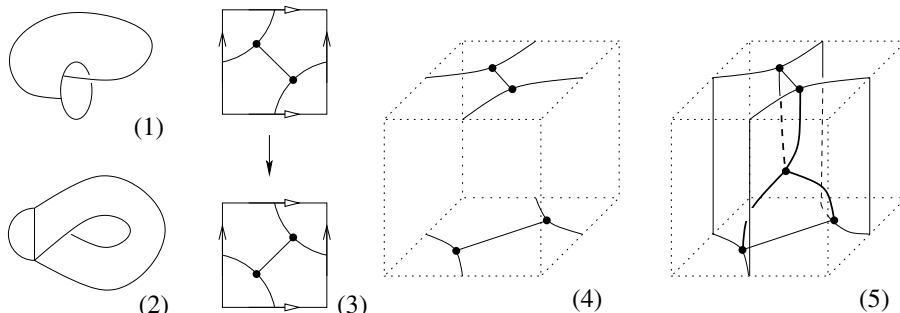
Figure 6: Two spines of the solid torus (1,2) and a flip (3,4) realized by adding a vertex (5).
