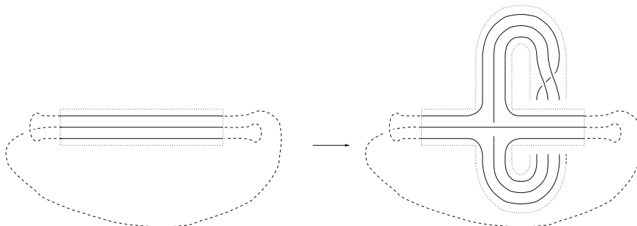
Figure 14: Left: attaching circle of the face outside an edge where it passes three times but not in the same direction. Right: a spine with one face and one more vertex.
