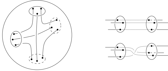
Figure 2: A tangle in a ball (left); a positive and a negative gluing of tangles (right).
