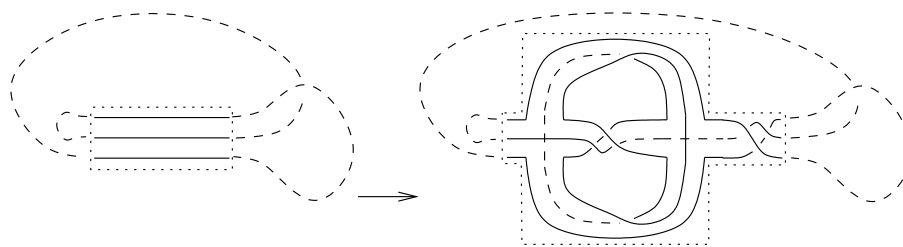
Figure 16: How to transform a spine of M \in \mathcal{M}_{g,k} to a spine of M' \in \mathcal{M}_{g+1,k+1} .
