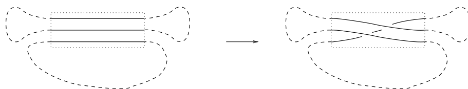
Figure 10: If a face passes twice with a counterpass, the number of faces can be reduced.
