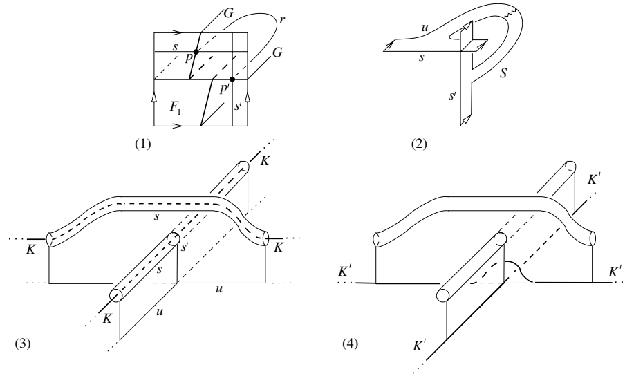
Figure 7: Isotoping a knot to 1-bridge position.
