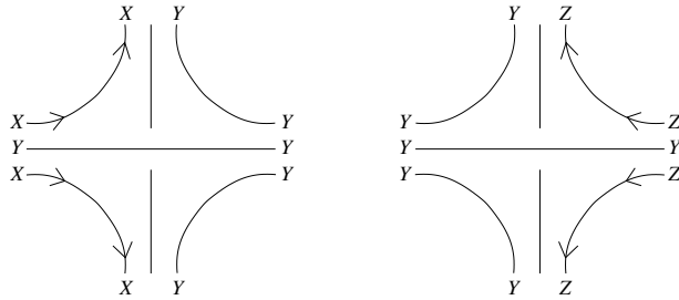
Figure 12: Conclusion of the proof.
