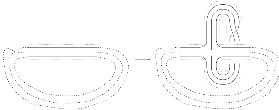
Figure 13: Left: attaching circles of faces outside an edge where a face passes twice. Right: a spine with one face and one more vertex.
