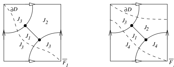
Figure 5: A slope in \{-1, 1/2, 1\} (left) or in \{-2, -1/2, 1/3, 2/3, 3/2, 3\} (right) is represented by a loop \partial D intersecting transversely S(P) \cap \overline{F_1} in two (left) or three (right) points.
