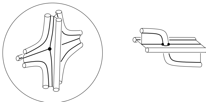
Figure 8: Portions of spine of the knot exterior.
