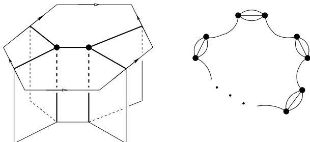
Figure 15: Spines of elements of \mathcal{M}_{g,g} .
