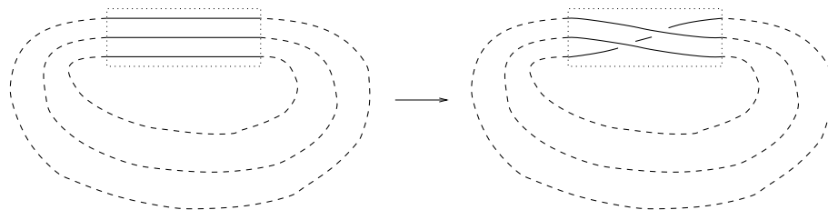
Figure 9: Left: if three different faces of P run along the edge e shown in the dotted box, their attaching circles in the rest of \partial U(S(P)) are connected as shown. Right: this modification of U(P) near e reduces the number of faces.
