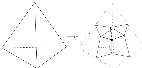
Figure 4: From an ideal triangulation to a standard spine.
