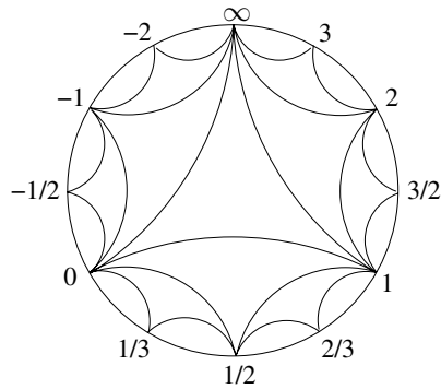
Figure 1: The Farey tessellation of \mathbb{H}^2 .
