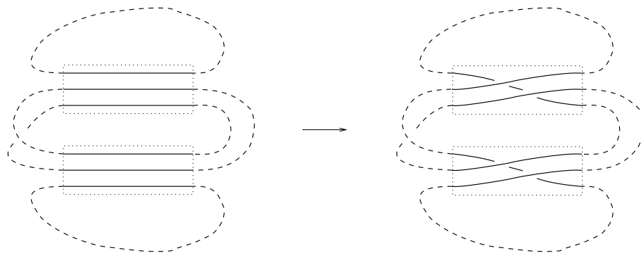
Figure 11: If a face passes twice along two edges with different companions, the number of faces can be reduced.
